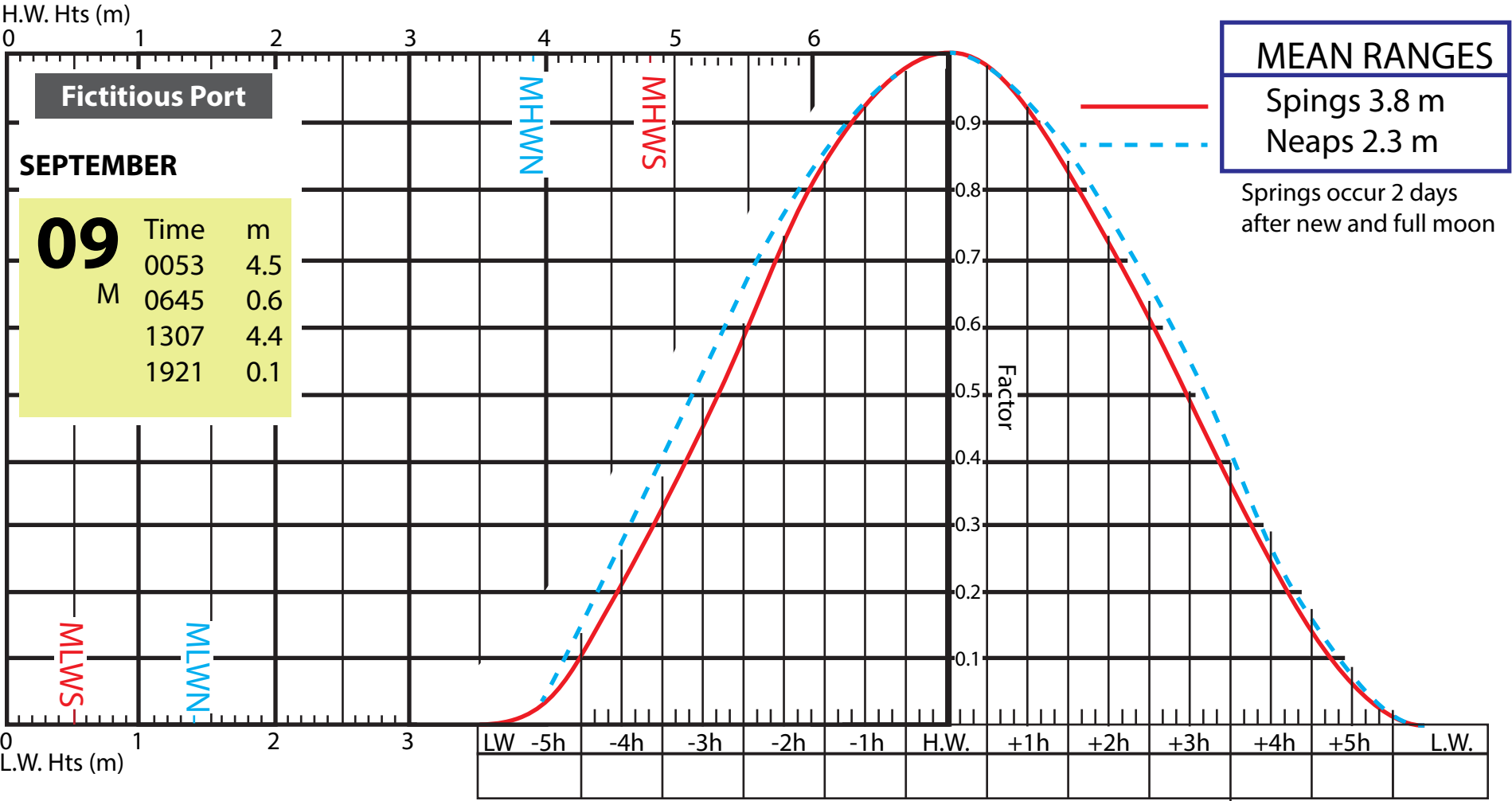
Typical Tidal Curve
